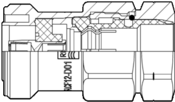
Cut 716F-LCF12-D01_DRW.PNG
