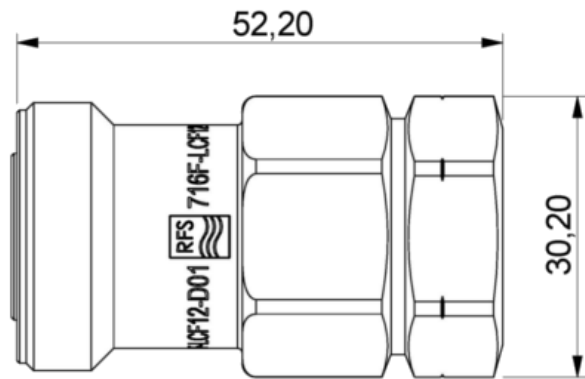
View 716F-LCF12-D01_DRW.PNG
